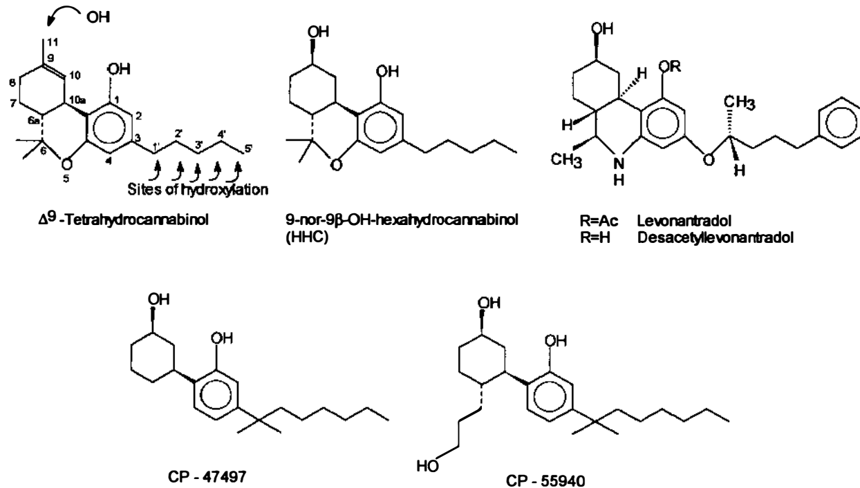
Figure 1 Structures of classical tricyclic and nonclassical bicyclic cannabinoid compounds.
